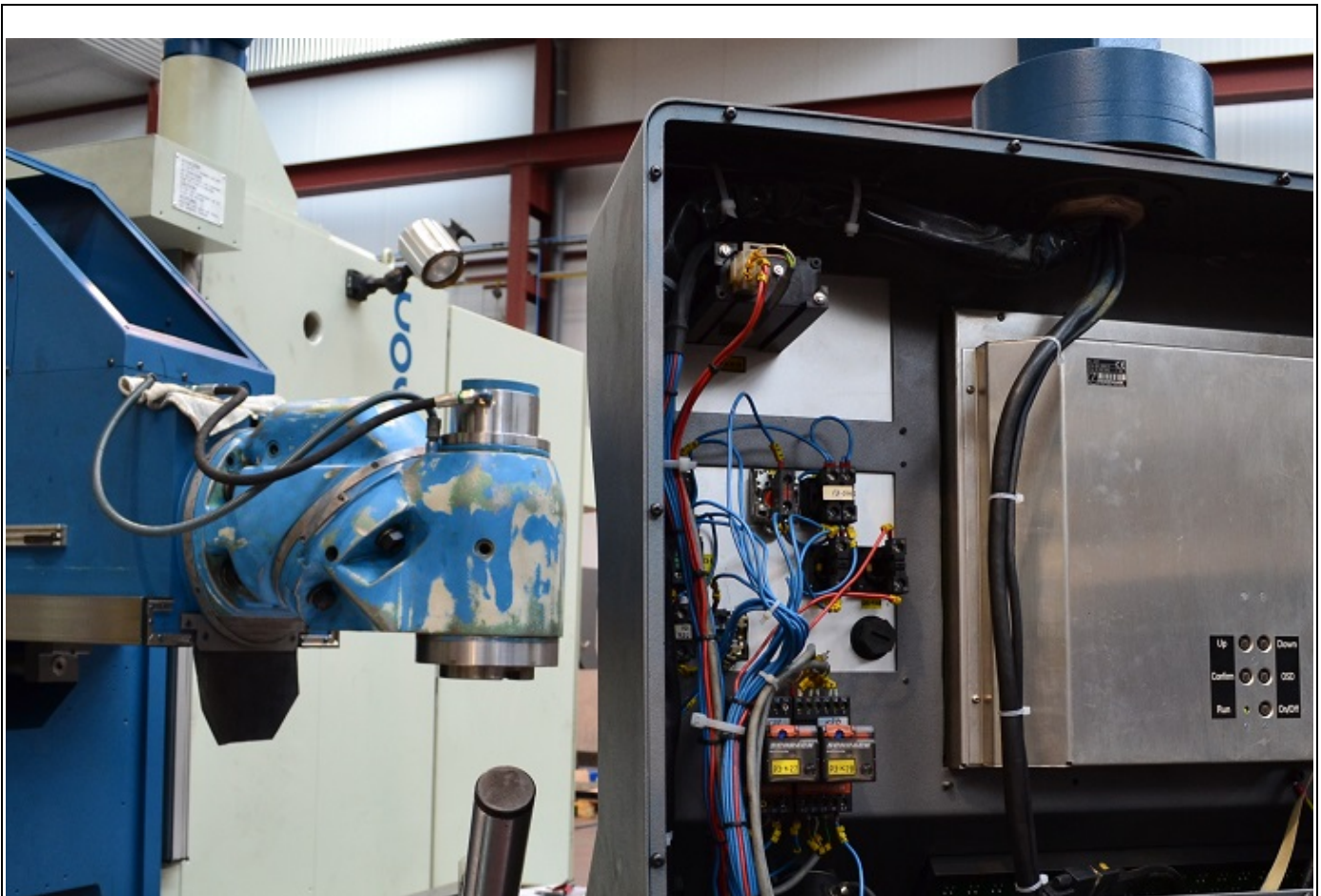
Milling machine CORREA CF 22/25
