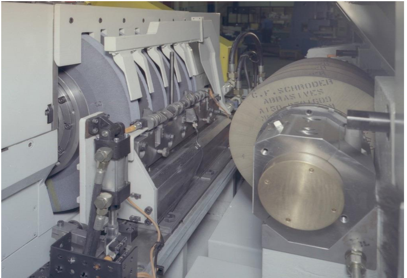
GIUSTINA R125.500 GRINDING MACHINE
